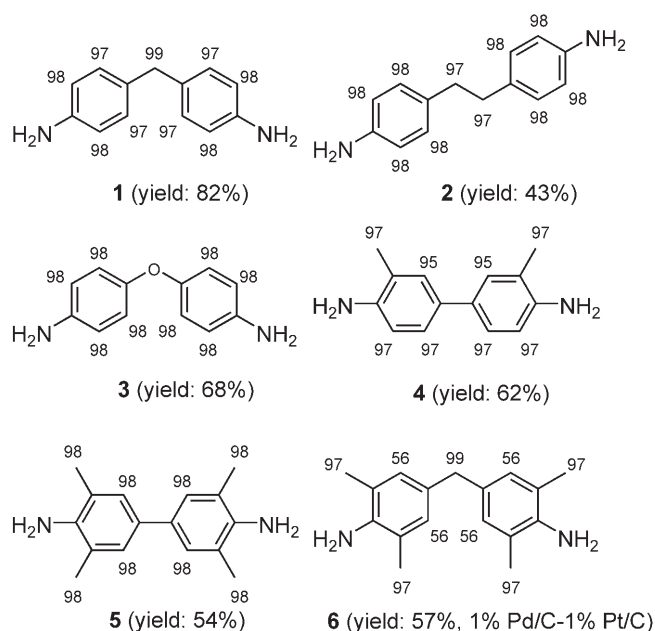
Figure 1. Deuteration of dianiline derivatives using the 10 % Pd/C–5 % Pt/C–D 2 O–H 2 system at 180 °C for 24 h.
